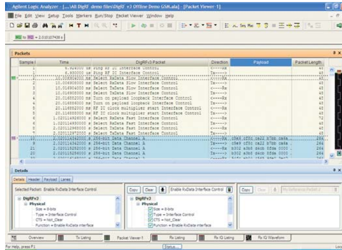
Packet view of DigRF traffic
